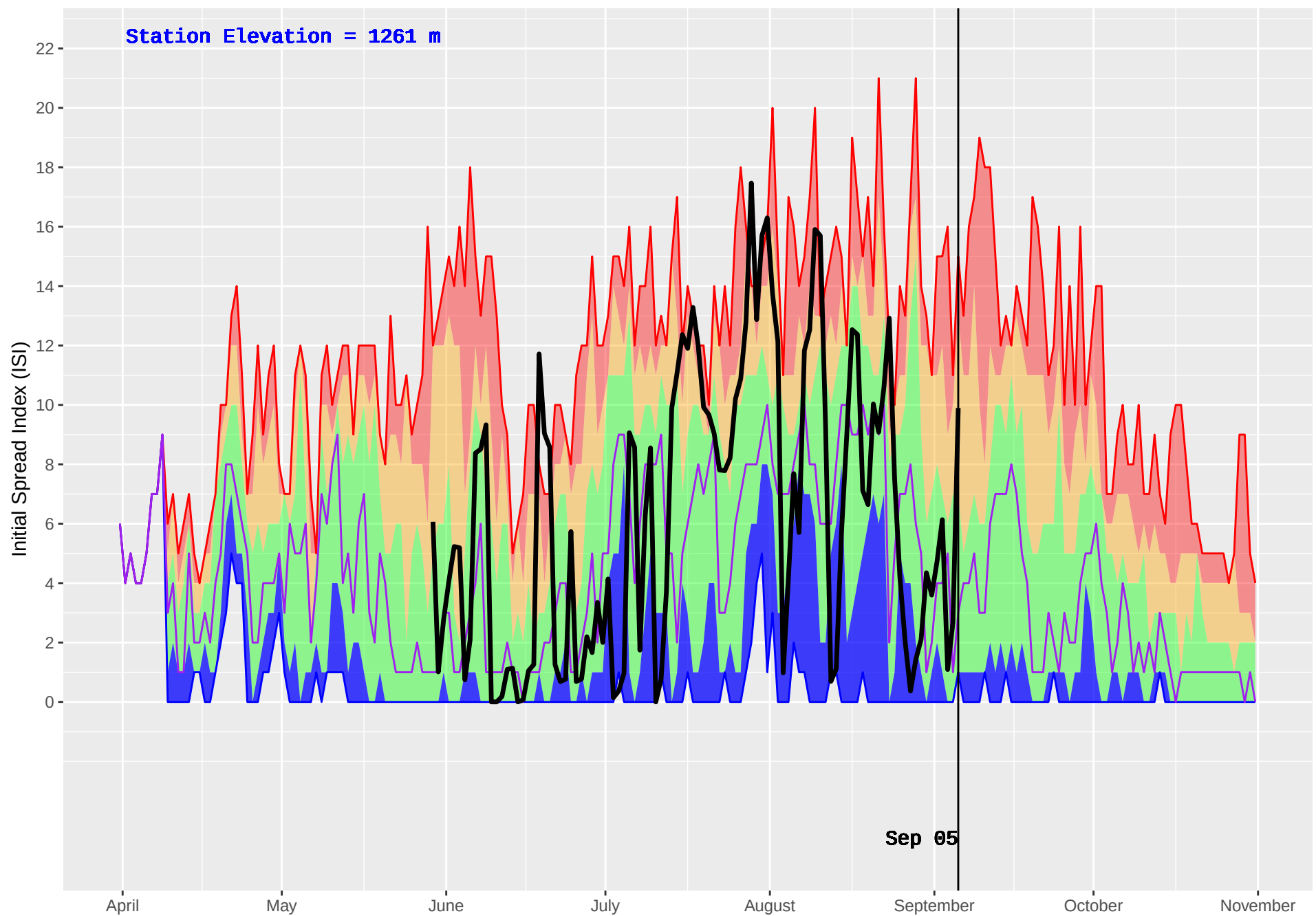
IDA BELL LAKE 3 (876) : Historical (2004–2016) and Current (2018) Daily Initial Spread Index (ISI)
