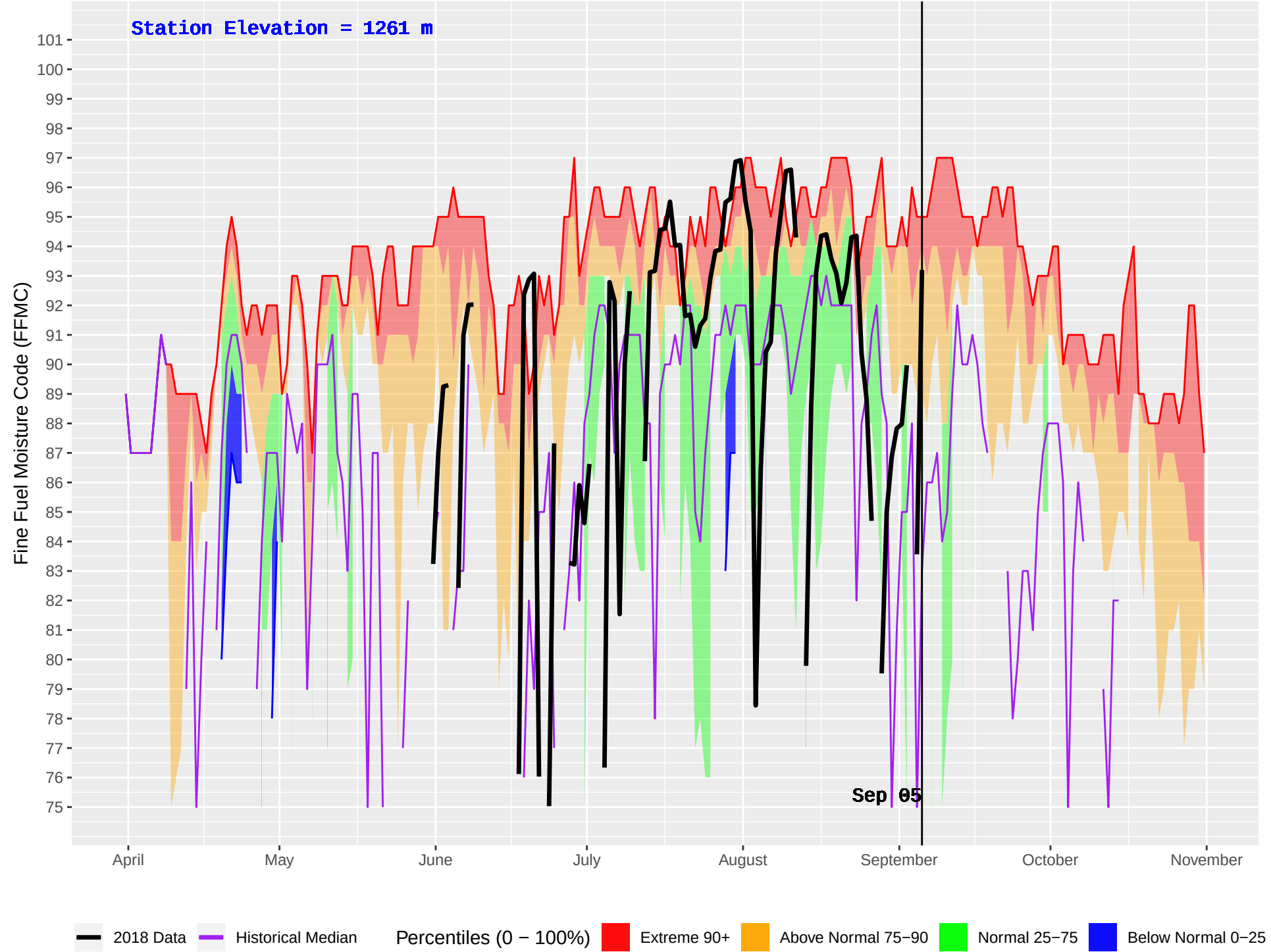
IDA BELL LAKE 3 (876) : Historical (2004–2016) and Current (2018) Daily Fine Fuel Moisture Code (FFMC)
