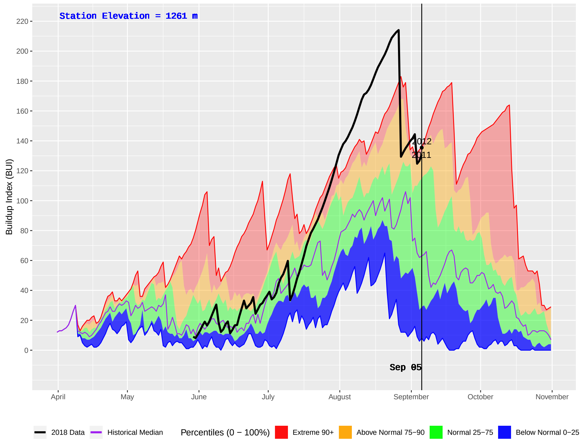
IDA BELL LAKE 3 (876) : Historical (2004–2016) and Current (2018) Daily Buildup Index (BUI)
