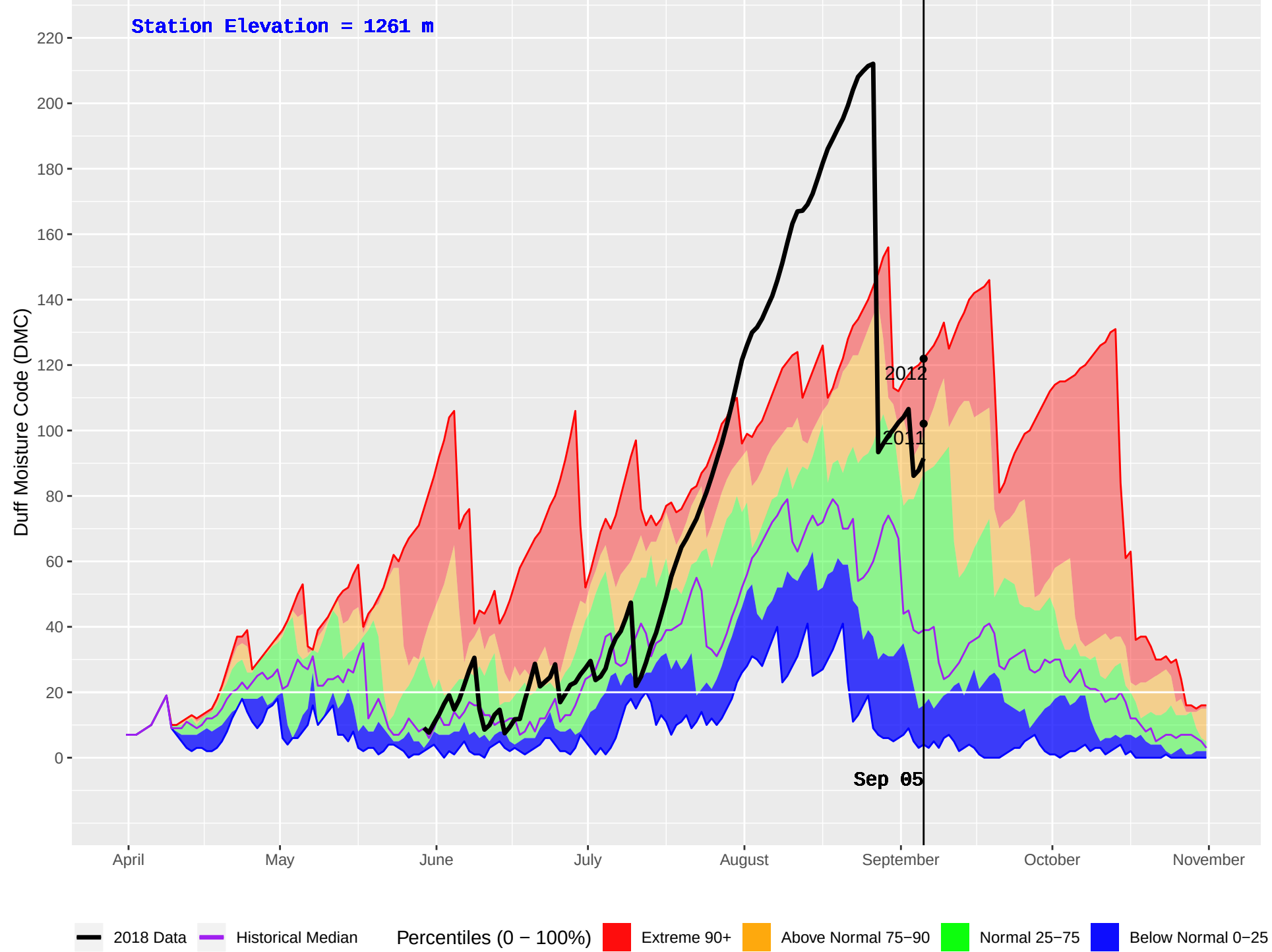
IDA BELL LAKE 3 (876) : Historical (2004–2016) and Current (2018) Daily Duff Moisture Code (DMC)
