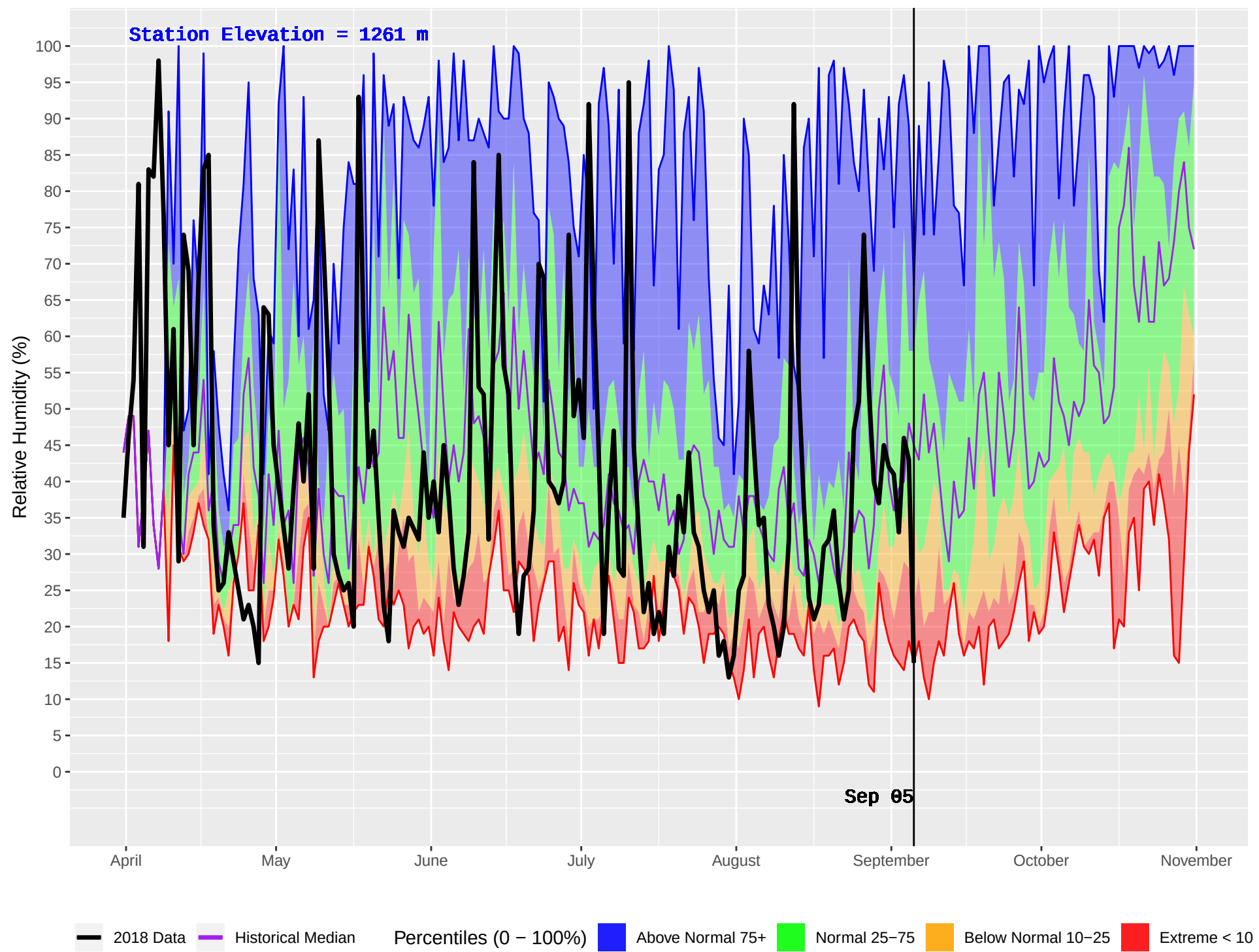
IDA BELL LAKE 3 (876) : Historical (2004–2016) and Current (2018) Daily Relative Humidity
