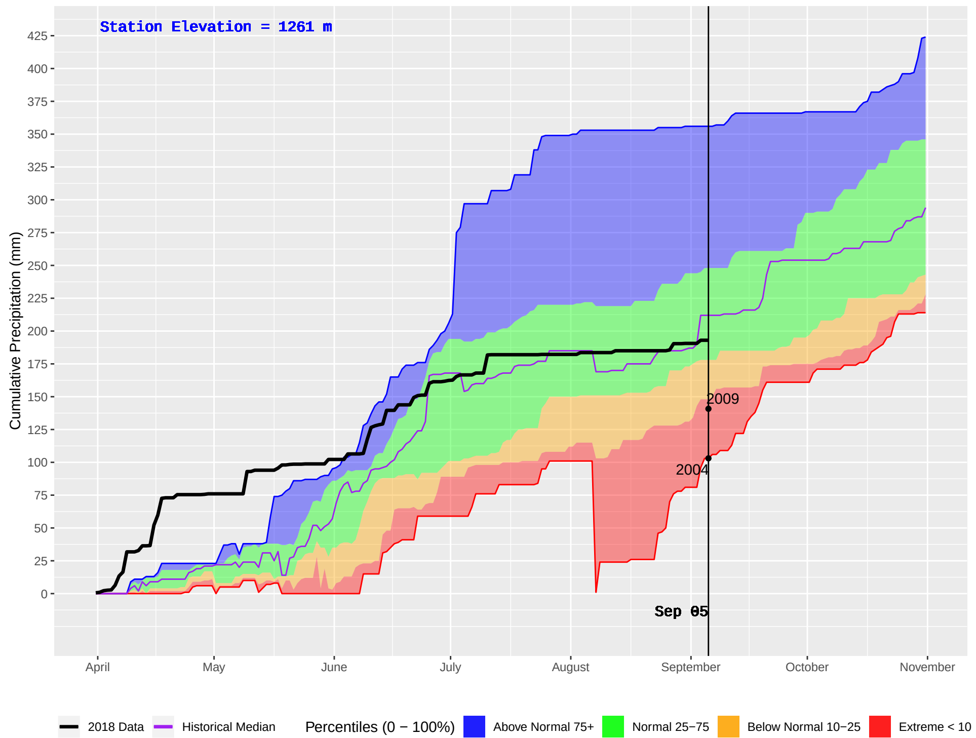
IDA BELL LAKE 3 (876) : Historical (2004–2016) and Current (2018) Daily Cumulative Precipitation
